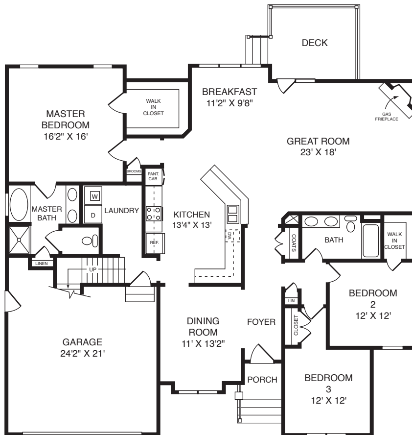
FIRST FLOOR
